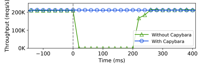
Figure 18: Throughput over time during server maintenance (starting at time 0). Capybara enables maintenance without service downtime.
