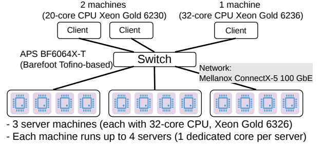
Figure 6: Evaluation cluster setup.
