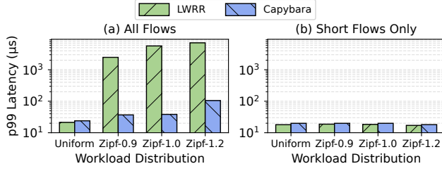
Figure 7: Skewed workloads increase LWRR’s p99 latency due to long-lived connections pinned to initial servers, while Cappybara mitigates this through dynamic connection migration.
