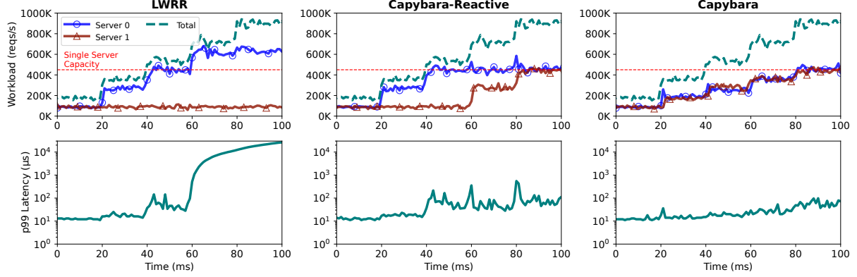
Figure 8: Capybara enables dynamic workload rebalancing across servers: the reactive policy quickly resolves server overload when it occurs, while the proactive policy prevents overload by continuously maintaining balanced workloads.
