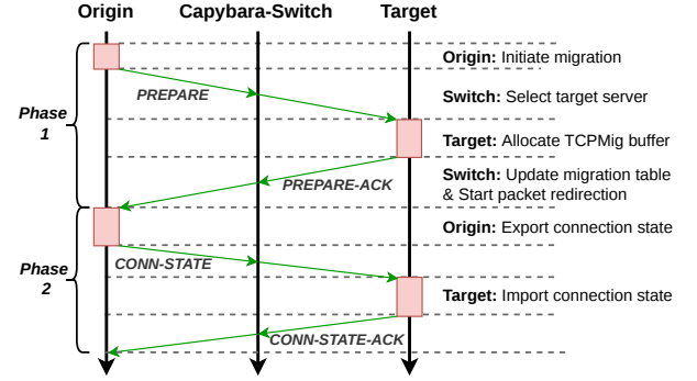
Figure 4: Cappybara two-phase migration protocol in action.
